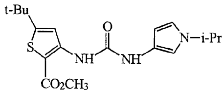
5-tert-Butyl-3-[3-(1-isopropyl-1H-pyrrol-3-yl)-ureido]-thiophene-2-carboxylic acid methyl ester
